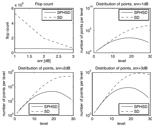
Fig. 1. Spherical relaxation for m = 30
