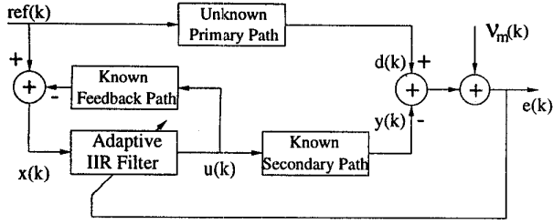
Fig. 1: Block Diagram of an ANC Problem With Feedback Contamination of the Reference Signal
