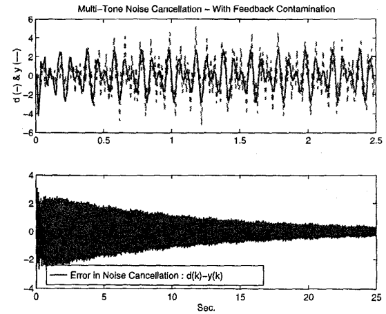
Fig. 5: The performance of the adaptive IIR filter when the reference signal is in the presence of feedback contamination. Note that for clarity, y(k) and d(k) are plotted for only 2.5 seconds.
