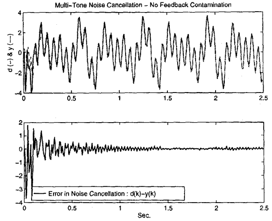
Fig. 4: The performance of the adaptive IIR filter in cancellation of the output of the secondary without feedback contamination
