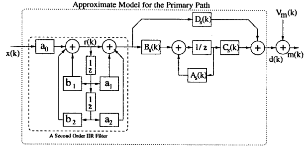
Fig. 3: Approximate Model For the Unknown Primary Path (A second order IIR filter is shown here)
