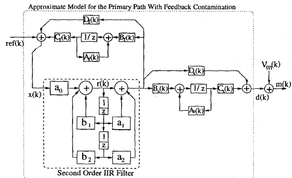
Fig. 6: Block diagram of the approximate model for the primary path in the presence of the feedback path
