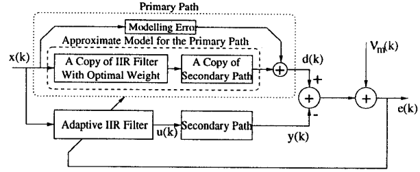
Fig. 2: Estimation Interpretation of the IIR Adaptive Filter Design in a ANC Problem
